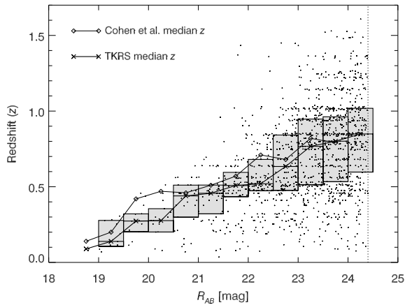
FIG. 15.— Redshift vs. R magnitude for targets with secure redshifts. Small pluses indicate individual objects in the TKRS survey. Boxes indicate the interquartile range of redshifts within respective 0.5 mag bins; each has a horizontal line and \times which indicate the median redshift within that bin. The median redshifts of Cohen et al. (2000) are shown for comparison. The vertical dotted line at right represents the apparent magnitude limit of the present survey at R_{AB} = 24.4 .
